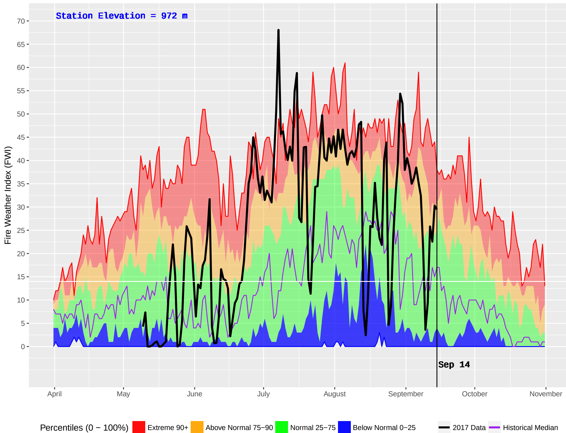
SPARKS LAKE (305) : Historical (1991–2016) and Current (2017) Noon Fire Weather Index (FWI)
